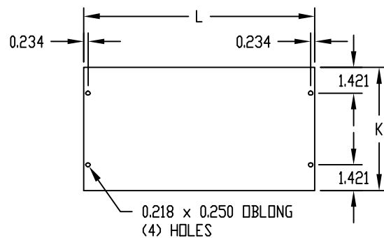
REAR PANEL
